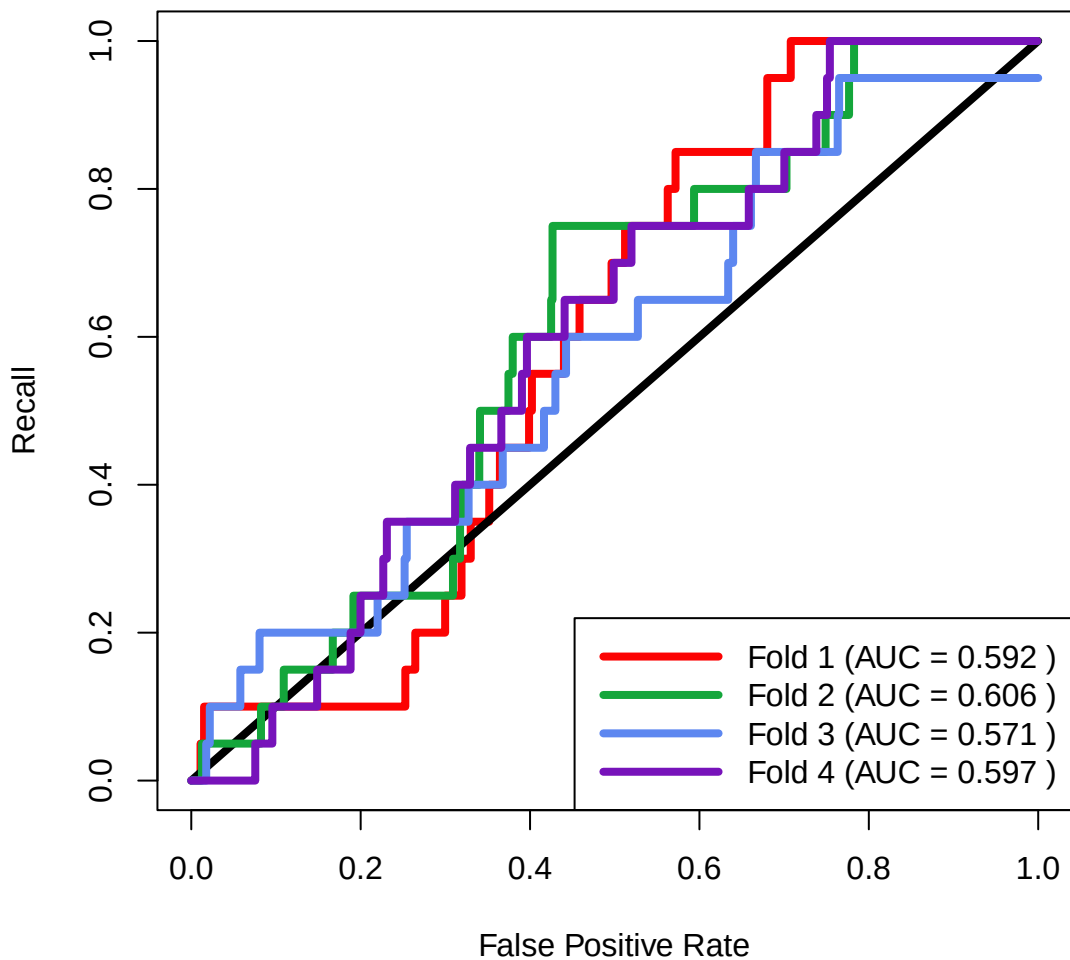
Primig2000: 24x20x8x1 Validation
